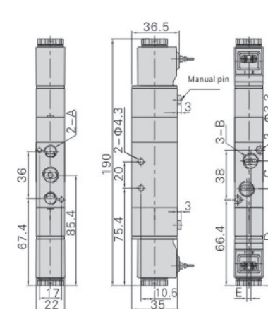
4V230 Outlet type
