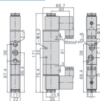
4V220DIN socket type
