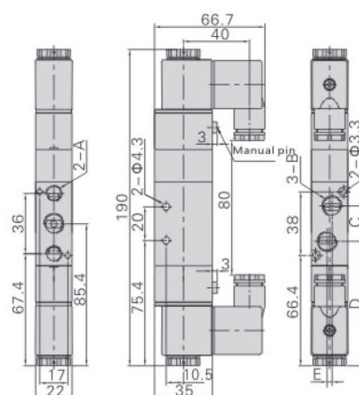
4V230DIN socket type
