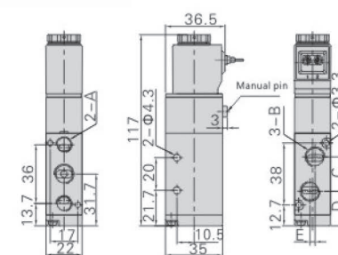
4V210 Outlet type
