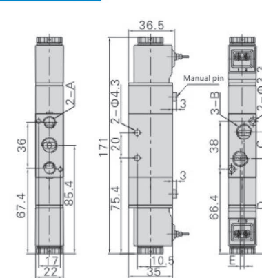
4V220 Outlet type
